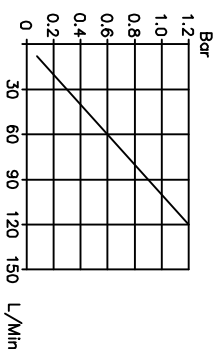
LOSS OF PRESSURE DIAGRAM
