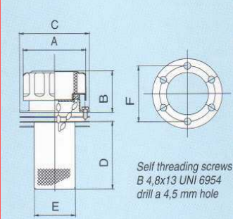
FILLER BREATHER
